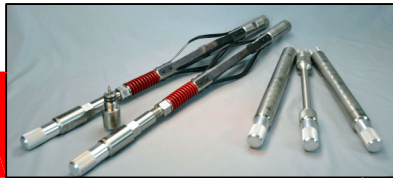
FPT ANCHOR OPTIONS (BOWSPRINGS & MAGNETS)
